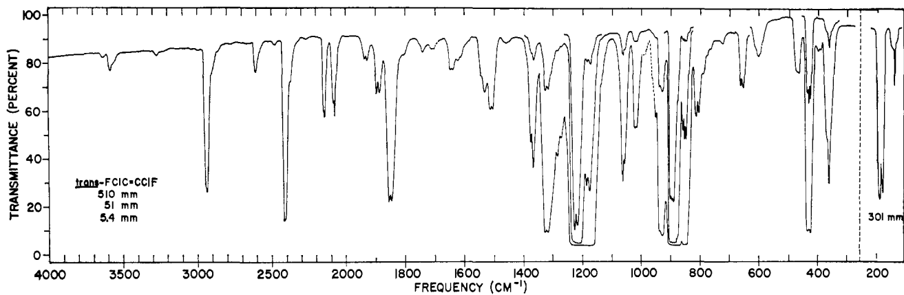
Figure 2. Gas phase infrared spectrum of trans -CFC1CFCl.
