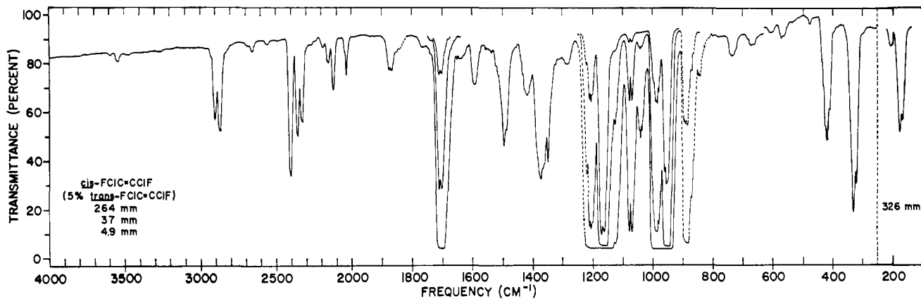
Figure 3. Gas phase infrared spectrum of cis -CFC1CFCl.
